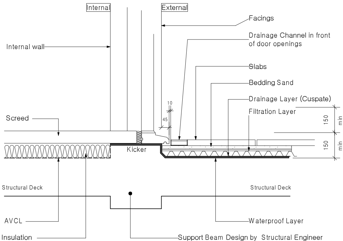
Podium deck - Threshold waterproofing detail (Bedded paviers)
