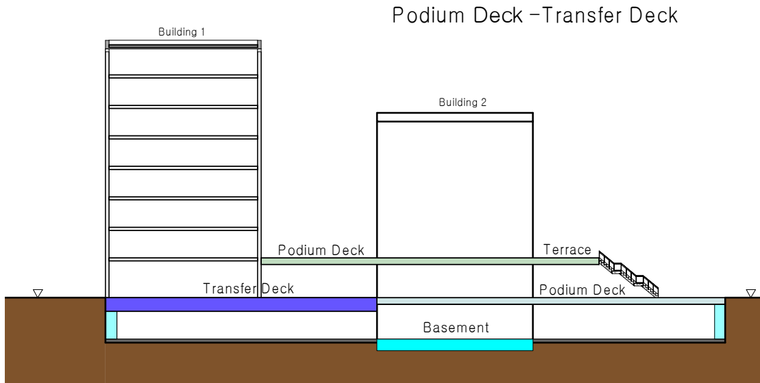
Typical podium deck and transfer deck examples
