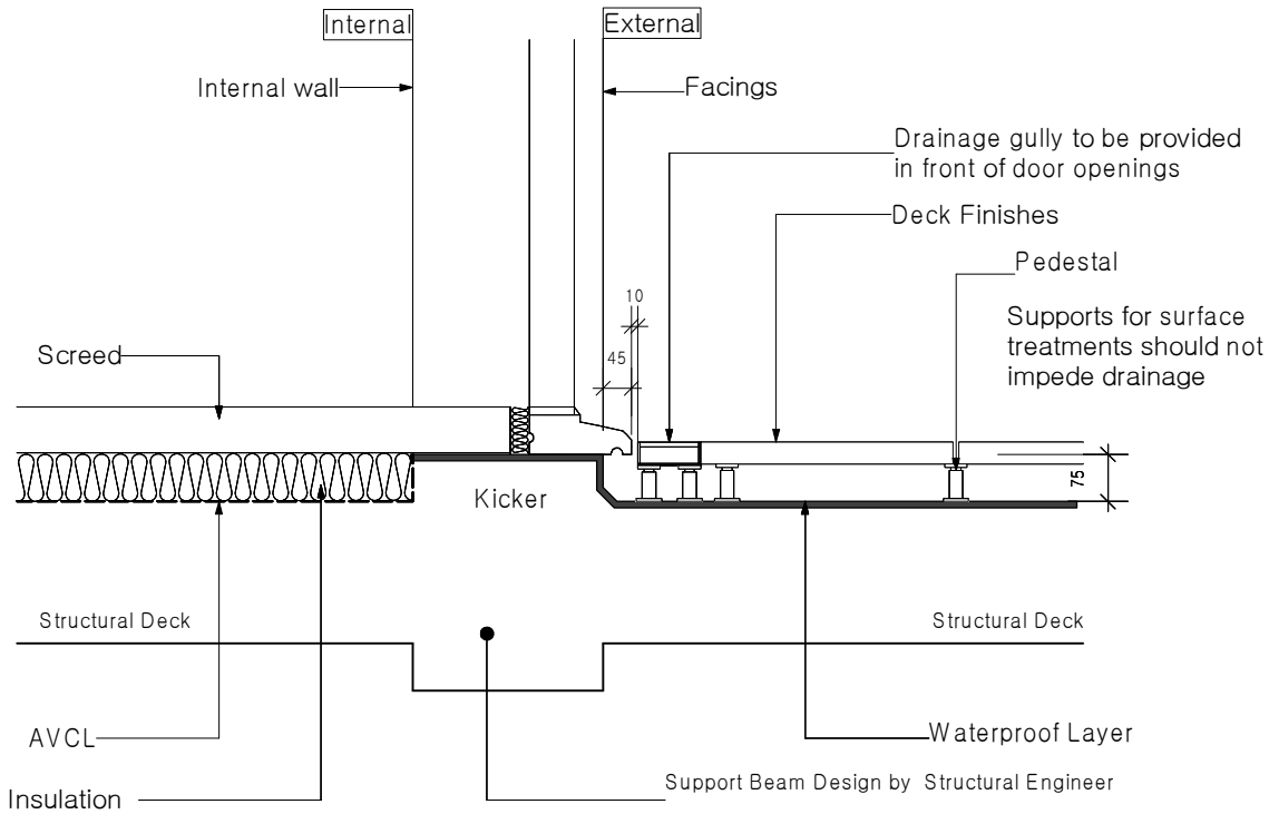
Podium deck - Threshold waterproofing detail (Slabs on pedestals)
