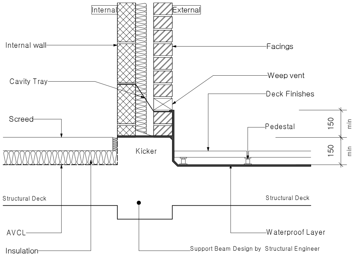
Podium deck – wall waterproofing detail (Slabs on pedestals)
