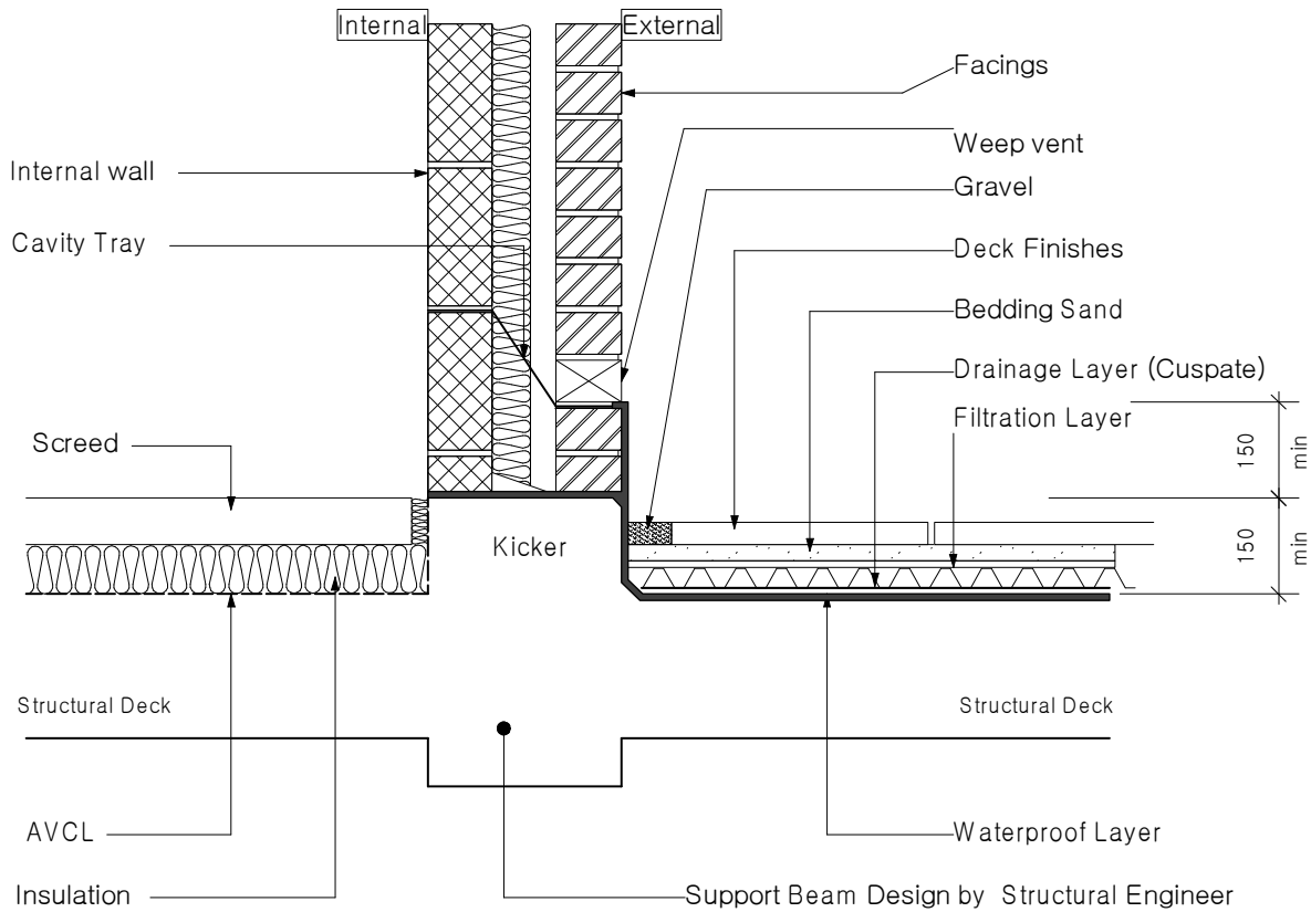
Podium deck – wall waterproofing detail (Bedded slabs)
