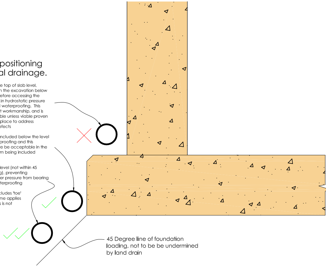
Figure 1: Suitable position of land drains
