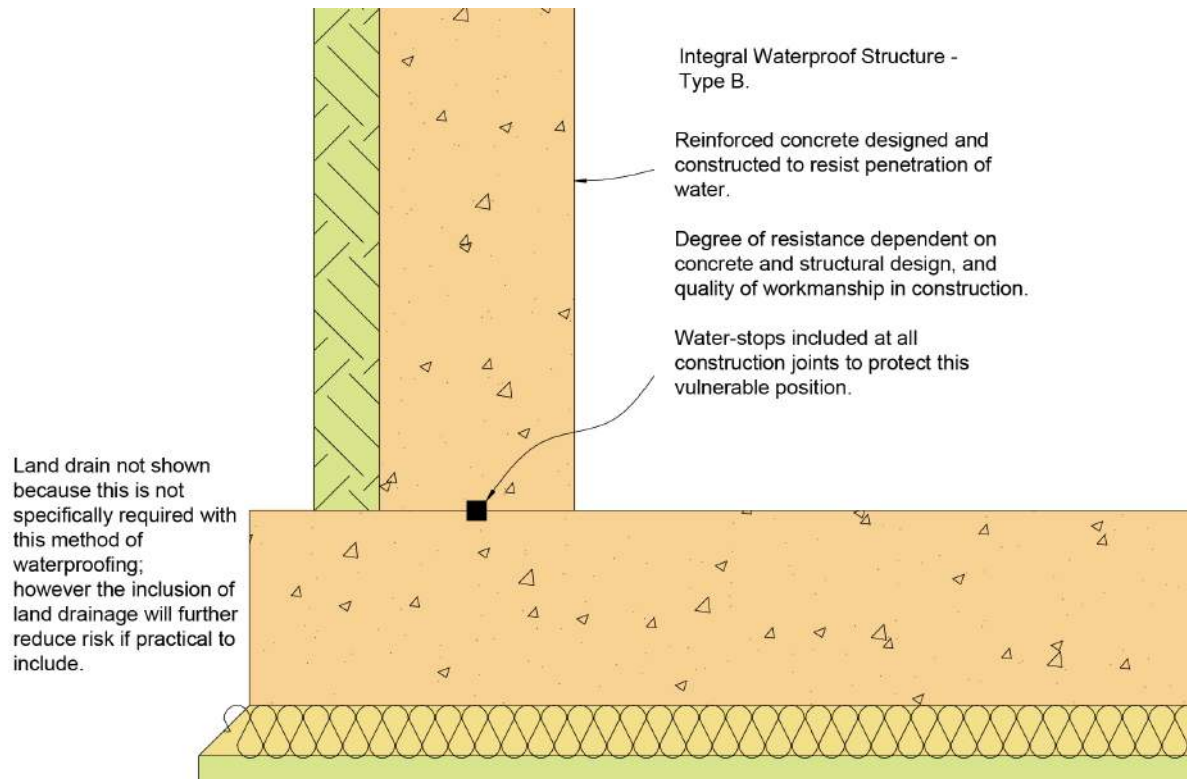
Figure 3: Type B, structurally integral protection
