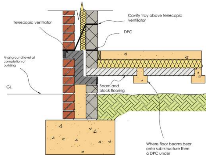
Figure 15: Typical precast beam and block floor without DPM
