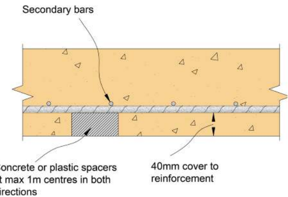
Figure 11: Cast in-situ suspended concrete floor - reinforcing cover and support
